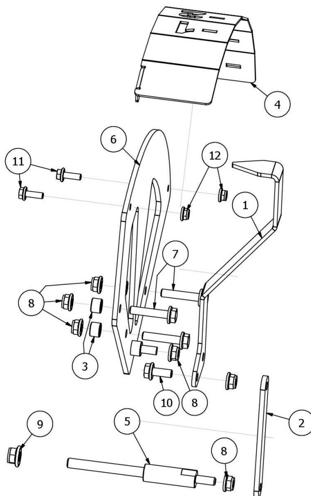
Rys. 18 AP02327 Skala Runner 30
