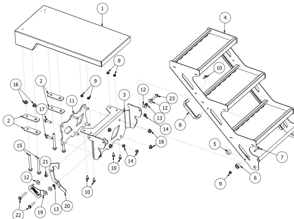
Rys. 18 AP02705 Schody z podestem RUNNER 35
