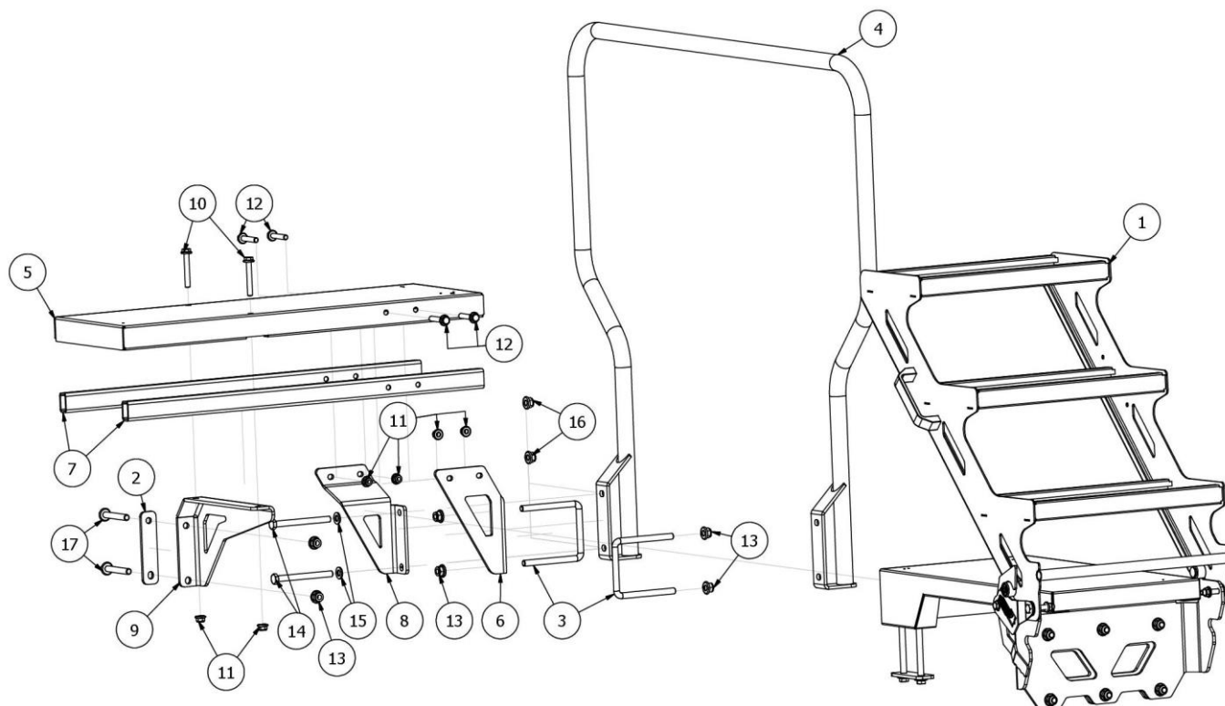
Rys. 17 AP02709 Schody z podestem RUNNER 35
