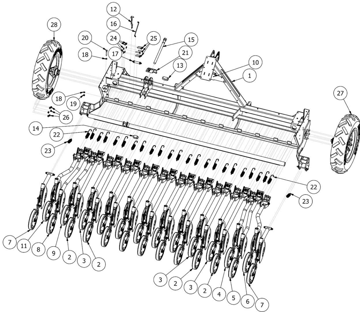
Rys. 3 SI01100 Rama z redlicami TC (25 redlic)
